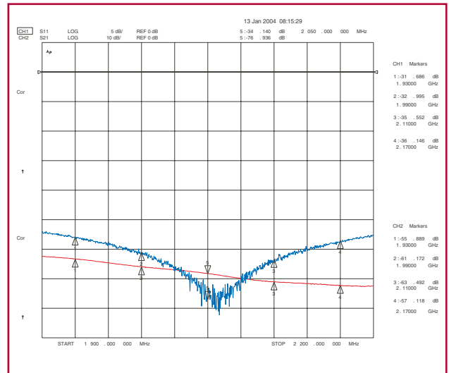
PCS/UMTS 20 dB Isolation
