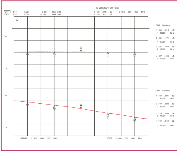
PCS/UMTS 20 dB Coupling
