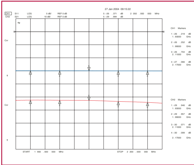
PCS/UMTS 30 dB Coupling
