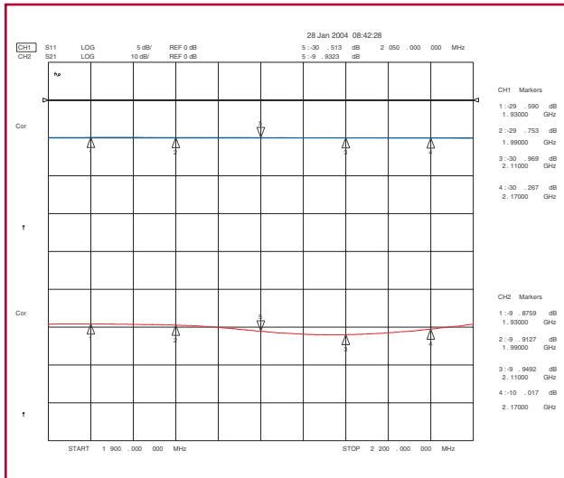
PCS/UMTS 10 dB Coupling
