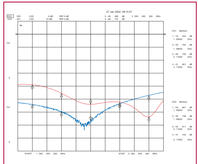
PCS/UMTS 30 dB Isolation
