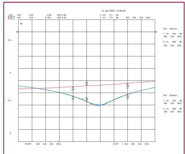
AMPS 20 dB Isolation
