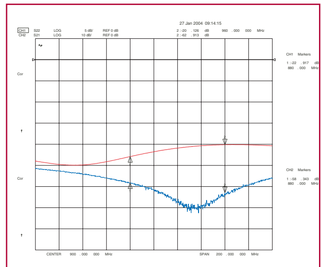
AMPS 30 dB Isolation
