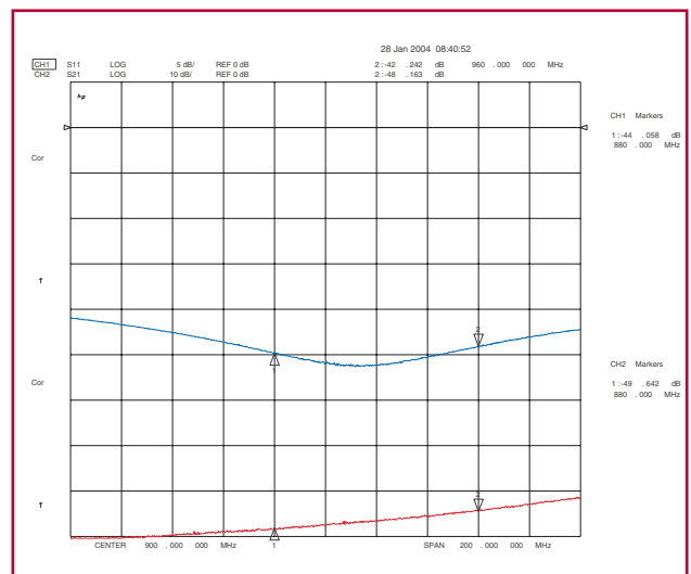
AMPS 10 dB Isolation
