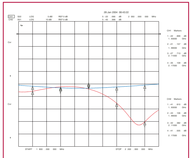
PCS/UMTS 10 dB Isolation
