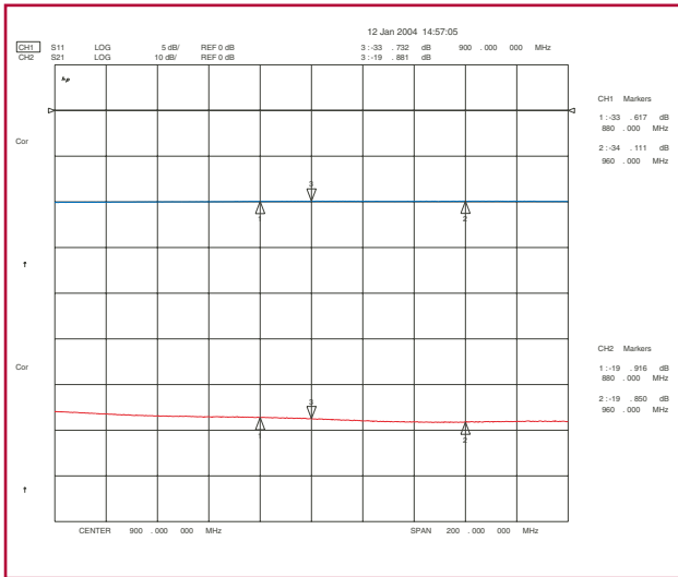
AMPS 20 dB Coupling
