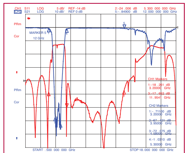
Passband Performance
