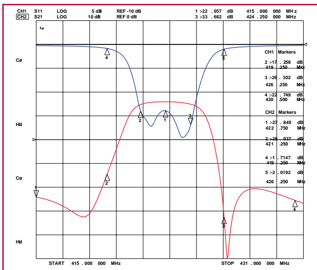
Passband Performance
